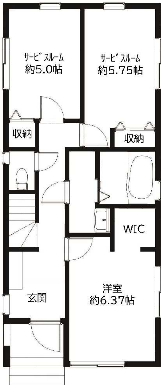
1F
